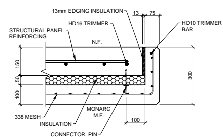
INSULATED PANEL ~ EXPOSED END DETAIL SCALE 1:20
