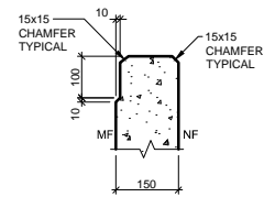
FLASHING DETAIL PANEL TOP SCALE 1:20
