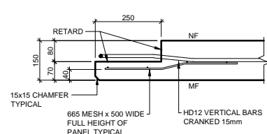
STITCH JOINT DETAIL SCALE 1:20
