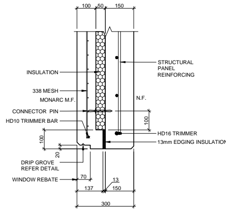
INSULATED PANEL ~ WINDOW REBATE DETAIL 1 SCALE 1:20
