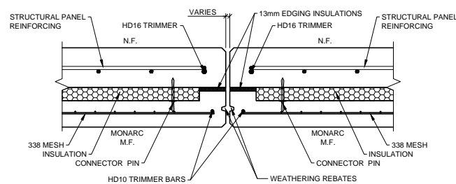
INSULATED PANEL TO PANEL DETAIL ~ STRAIGHT JOINT SCALE 1:20
