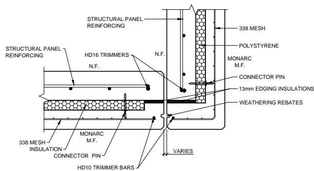
INSULATED PANEL TO PANEL DETAIL ~ CORNER JOINT SCALE 1:20
