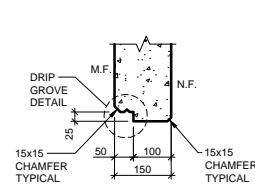
HEAD DETAIL SCALE 1:20
