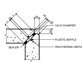
NAUHRIA MITRED CORNER DETAIL SCALE 1:20
