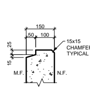
SILL DETAIL SCALE 1:20
