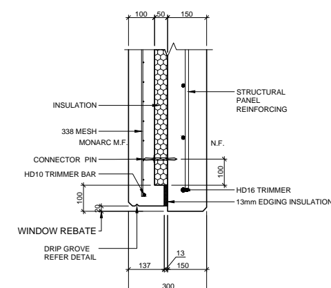
INSULATED PANEL ~ WINDOW REBATE DETAIL 2 SCALE 1:20
