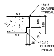
JAM DETAIL SCALE 1:20
