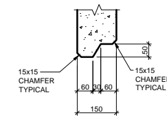
WEATHERING DETAIL PANEL BOTTOM SCALE 1:20
