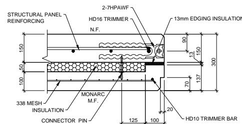
INSULATED PANEL ~ WINDOW REBATE DETAIL 1 SCALE 1:20
