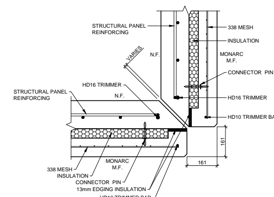
INSULATED PANEL TO PANEL DETAIL ~ MITRE JOINT SCALE 1:20
