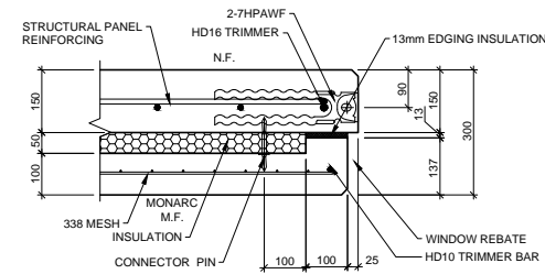
INSULATED PANEL ~ WINDOW REBATE DETAIL 2 SCALE 1:20
