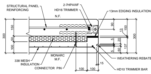
INSULATED PANEL ~ WEATHERING REBATE DETAIL SCALE 1:20
