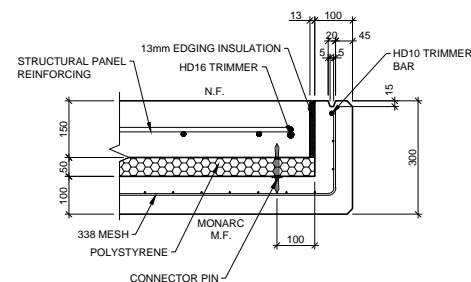
INSULATED PANEL ~ CORNER DETAIL SCALE 1:20
