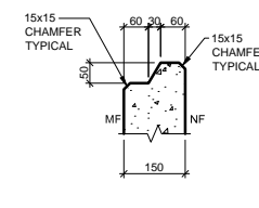
WEATHERING DETAIL PANEL TOP SCALE 1:20
