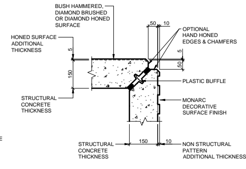
NAUHRIA CORNER DETAIL FOR MONARC PANEL SCALE 1:20
